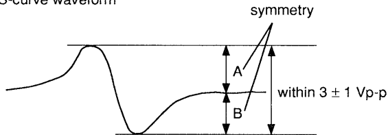
S-curve waveform
